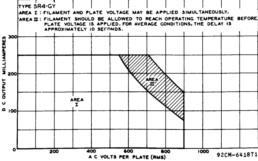
OPERATION CHARACTERISTICS WITH CAPACITOR INPUT TO FILTER
